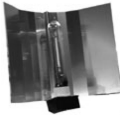
Figure 5.11 - This is an example of a HPS and also a MH Light system. There is nothing at face value to Indicate that the light is a HPS or a MH. To check this out we need to look at the ballast and the bulb and read what is says about the type of light system that it is. MH lights tend to give off a blue tone, while HPS tend to give off an orange tone.
